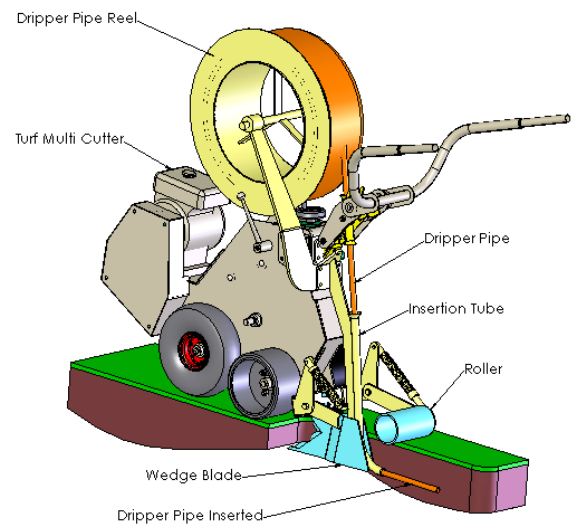
DRIP FEED IRRIGATION INSERTION USING THE WEDGE BLADE
